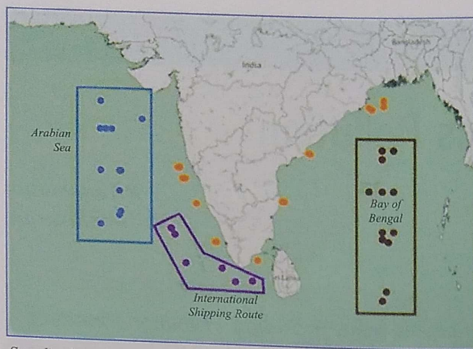
Sampling locations in Northern Indian Ocean for assessment of marine plastics
