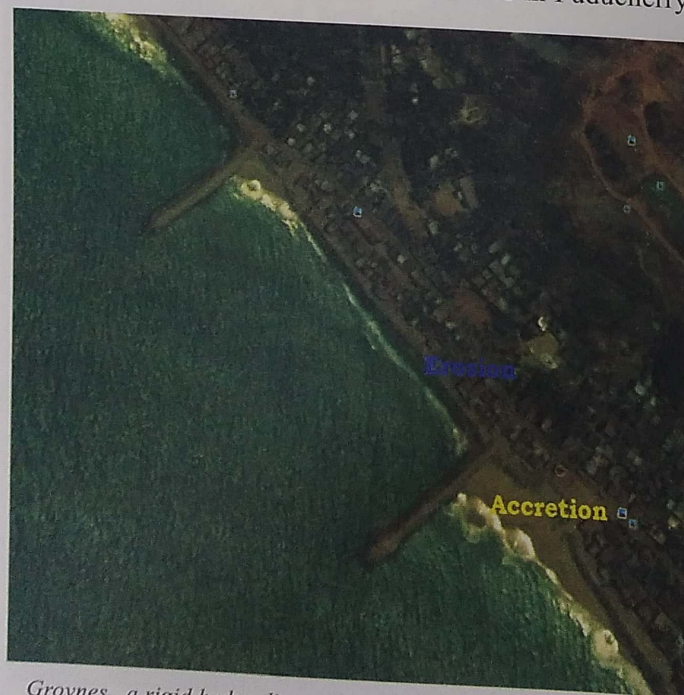
Groynes, a rigid hydraulic structure built perpendicularly from an ocean shore (in coastal engineering) or a river bank
