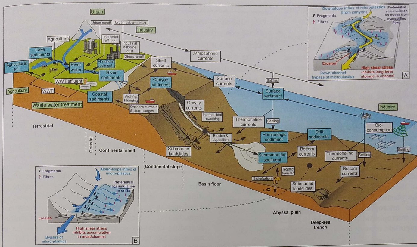
Settlement and transport of plastics in the midwater column of the ocean through various governing factors (Source : Kane & Clare, 2019)
